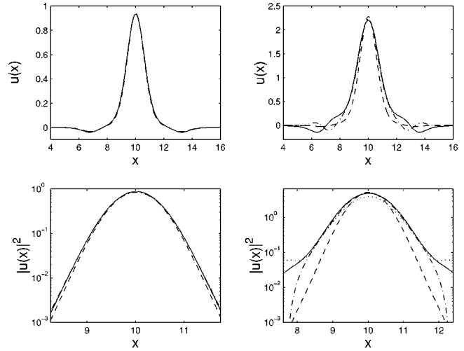
FIG. 1. Comparison of the lattice reconstructed solution in the tight-binding (dashed line) and the 3-band (dashed-dotted line) approximation with the numerical solution of the GP equation (14) (solid line). The comparison is performed for V(x) = -5 \cos(2x) and different chemical potentials: \mu = 1.5 (left panels) and \mu = -1.5 (right panels). The bottom panels show the same features as the top ones using semi-log plots. Additionally, in both the left and right bottom panels, there is a dotted line showing the result of the dynamical evolution (at t \approx 50 ), of the tight-binding approximation in the corresponding cases (i.e., \mu = -1.5 for the left panel and \mu = -1.5 for the right one.) In the left panel, the dynamical evolution practically coincides with the exact solution. In the right panel, the tight-binding initial condition tries to deform itself (from the dashed to dotted profile) to “approach” the shape of the exact solution (solid line).
