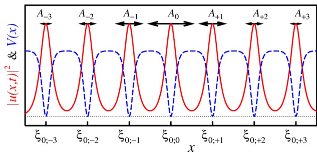
FIG. 2. (Color online). A quasi-1D condensate (solid line) in a deep periodic optical-lattice potential (dashed line). The condensate is effectively described as a chain of coupled solitons whose positions follow a Toda lattice with on-site potentials [Eq. (31)]. Using the oscillating ansatz (32), where the j th soliton is forced to oscillate with amplitude A_j , one can further reduce the dynamics to a second-order recurrence relationship between neighboring amplitudes [Eq. (33)].
